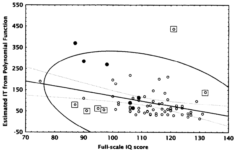
Fig. 7. Estimated IT vs Full-Scale IQ. The solid filled markers are those with the lowest percentage fit values as detailed in Table 5. The markers surrounded by a square correspond to those cases removed in order to maximise the IQ \times IT correlations. A 99% confidence ellipse is also plotted on this graph.
