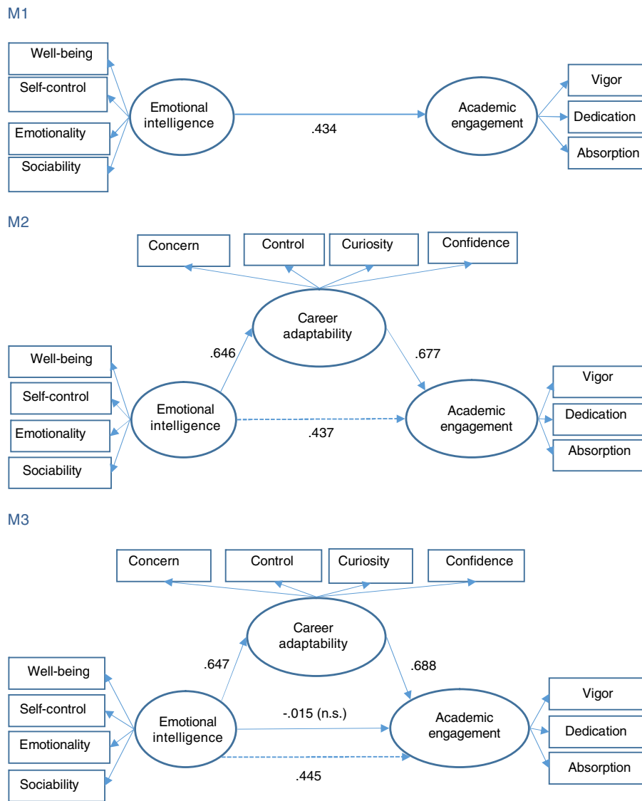
Figure 2. Steps of mediation analysis. M1: Total effect model, M2: Indirect effect model, M3: Indirect and direct effects model. \rightarrow : Indirect effects, \longrightarrow : Direct effects, n. s.: not significant.
